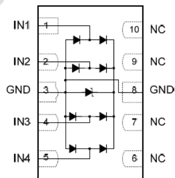
Circuit Diagram DFN-10 (Top-view)
